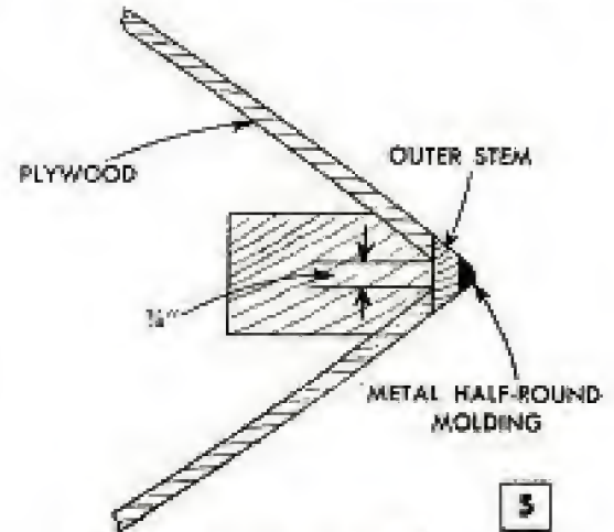
STEM CROSS SECTION
